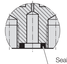
View/Design gas spring with flat seal
