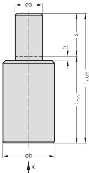
View/Design X - gas spring
