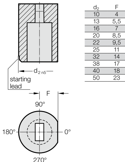
Anti-rotation element 4 (4)
