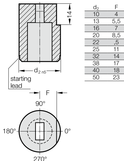
Anti-rotation element 5 (5)
