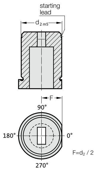
Anti-rotation element 4 (4)
