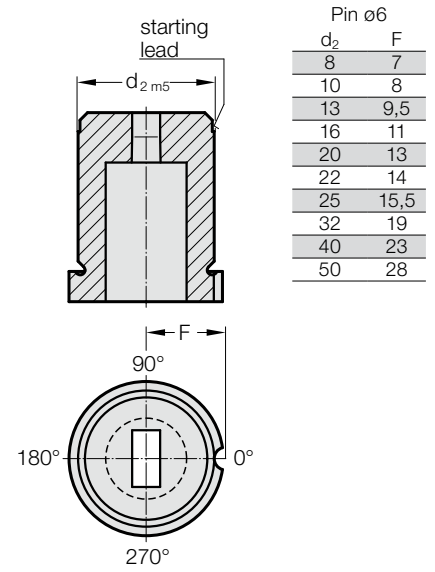
Anti-rotation element 3 (3)
