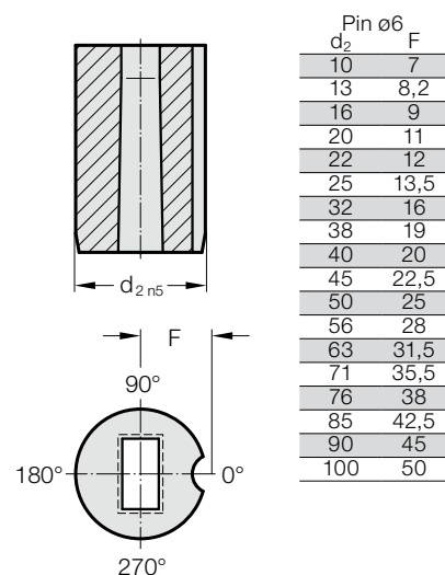
Anti-rotation element 3 (3)
