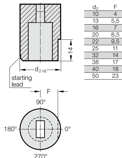
Anti-rotation element 6 (6)
