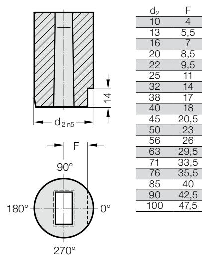
Anti-rotation element 6 (6)
