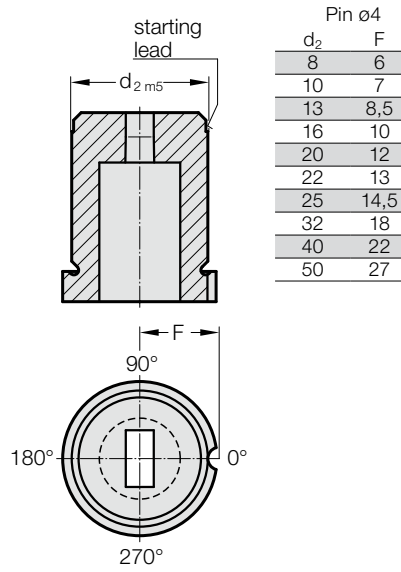
Anti-rotation element 2 (2)
